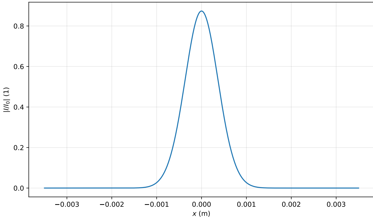
Intensity profile I(x, y = 0, z = 0.876m)/I_0 , P_{in}=0.1P_{cr} , artificial time
